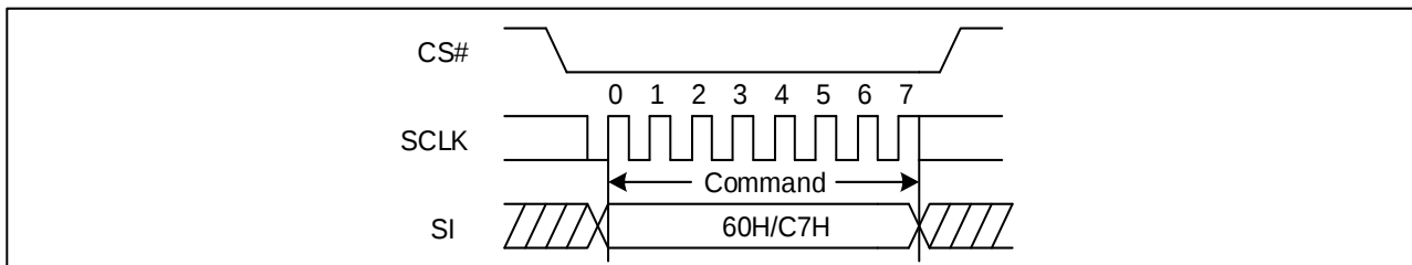
Figure 15. Chip Erase Sequence Diagram
