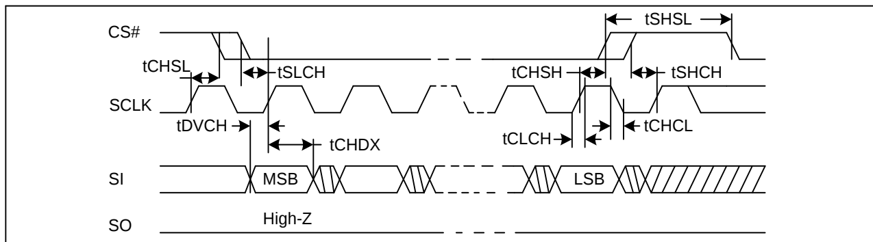
Figure 28. Input Timing
