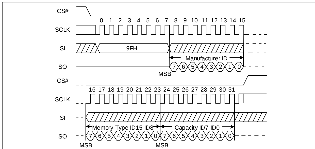
Figure 17. Read Identification ID Sequence Diagram
