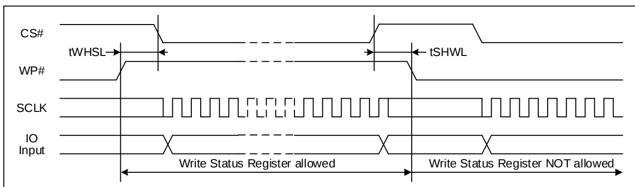
Figure 30. WP# Timing
